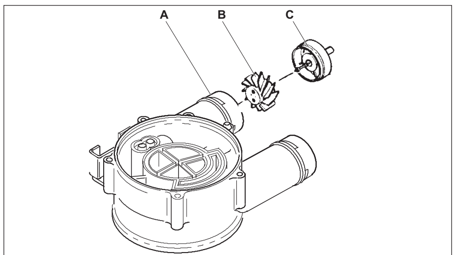
Abb. 9: Turbine
